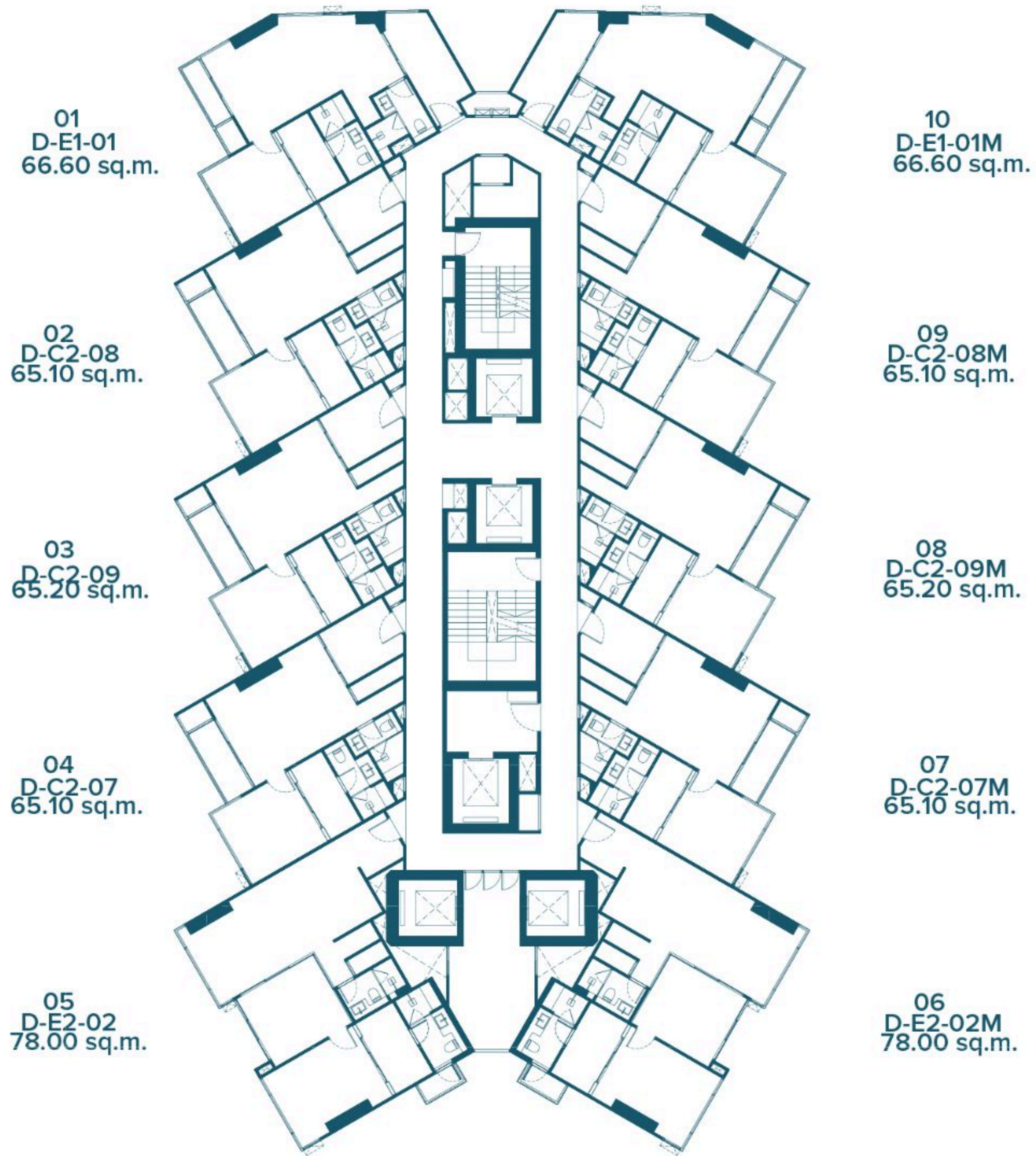
11th ,12Ath ,15th ,17th Floor Plan
