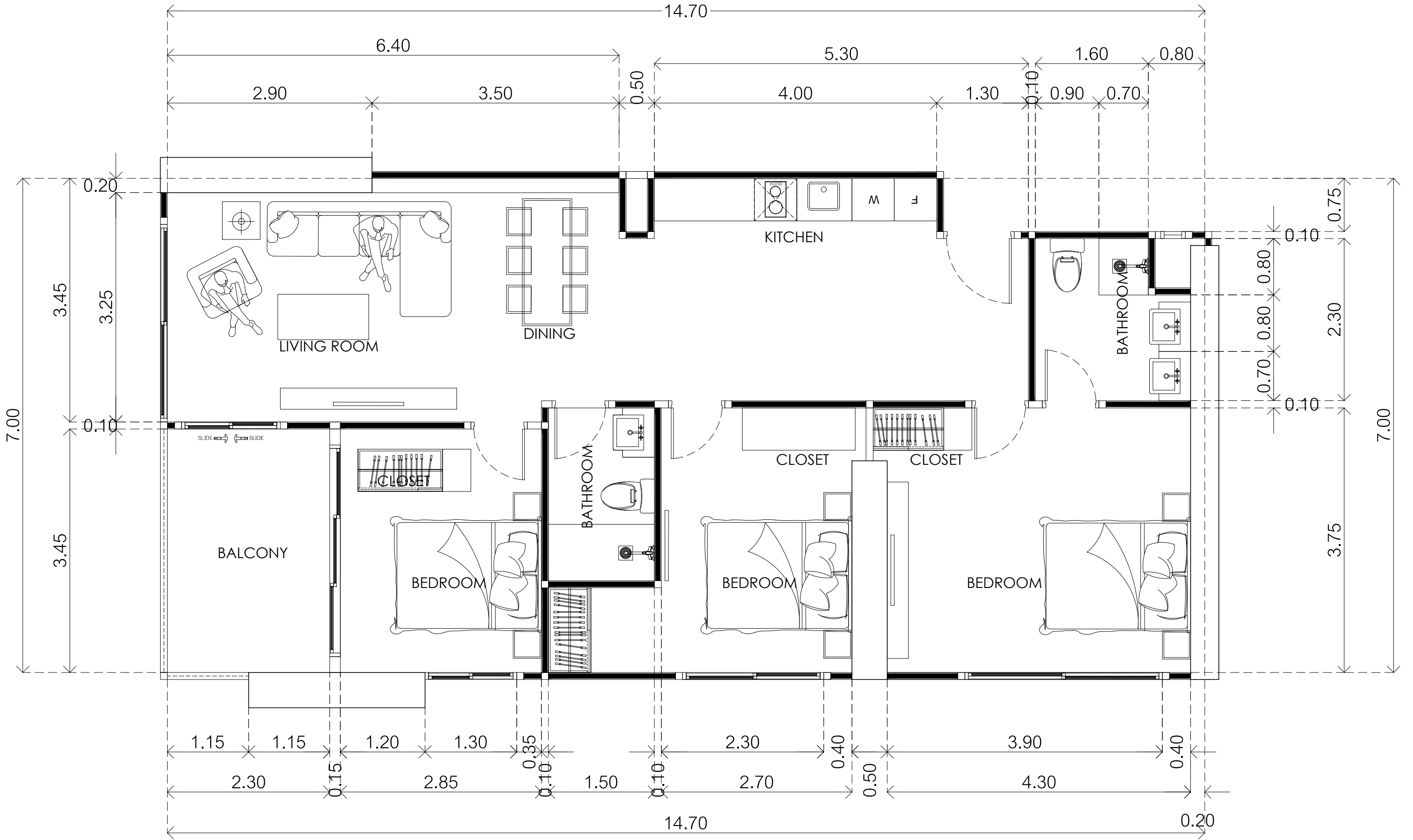
2BEDROOM 98.35 m 2 Scale 1:50
