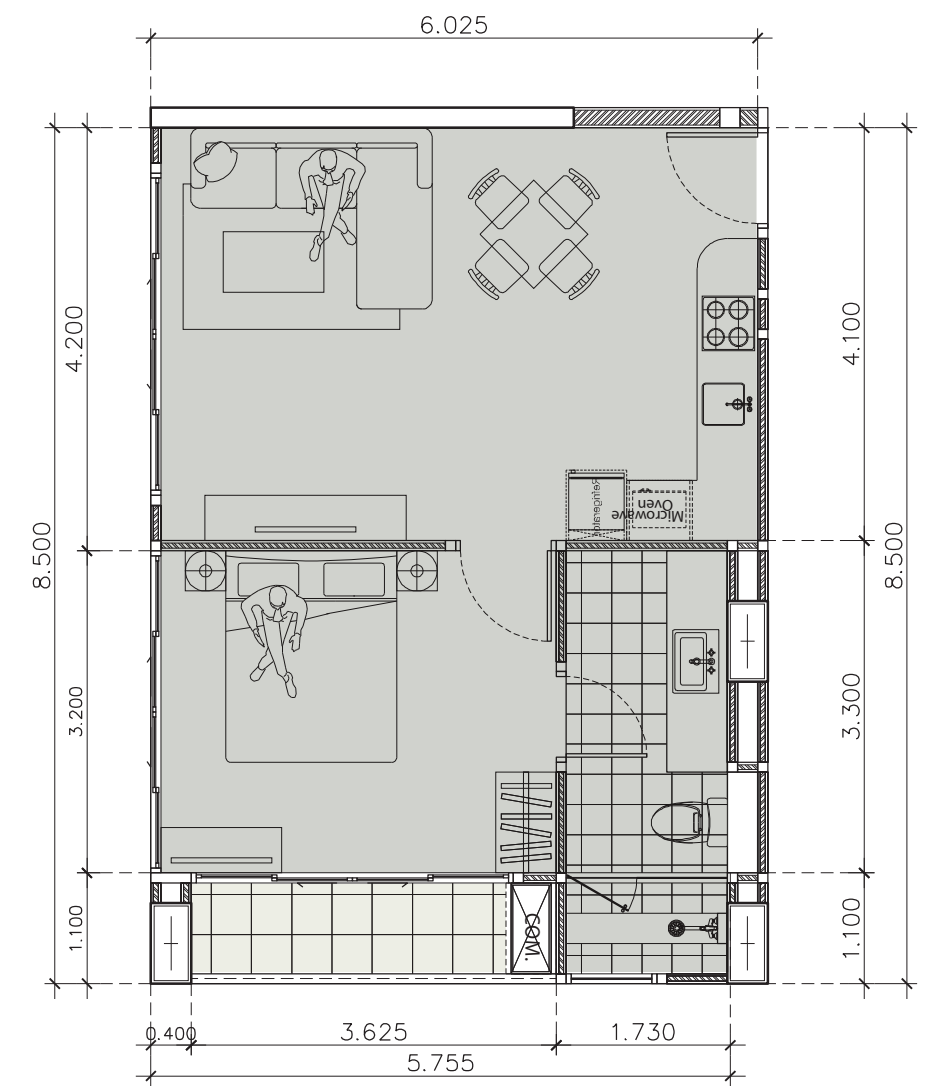
TYPE G 1 Bedroom DETAIL PLAN 50.51m 2
