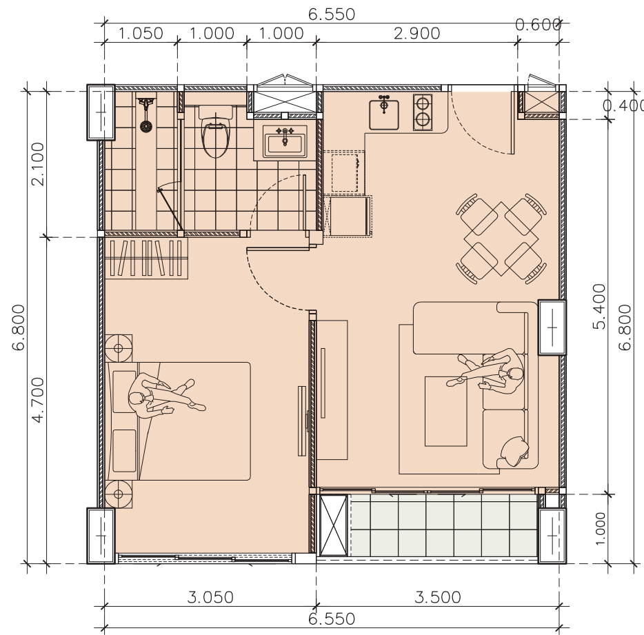
TYPE B 1 Bedroom DETAIL PLAN 43.25m 2
