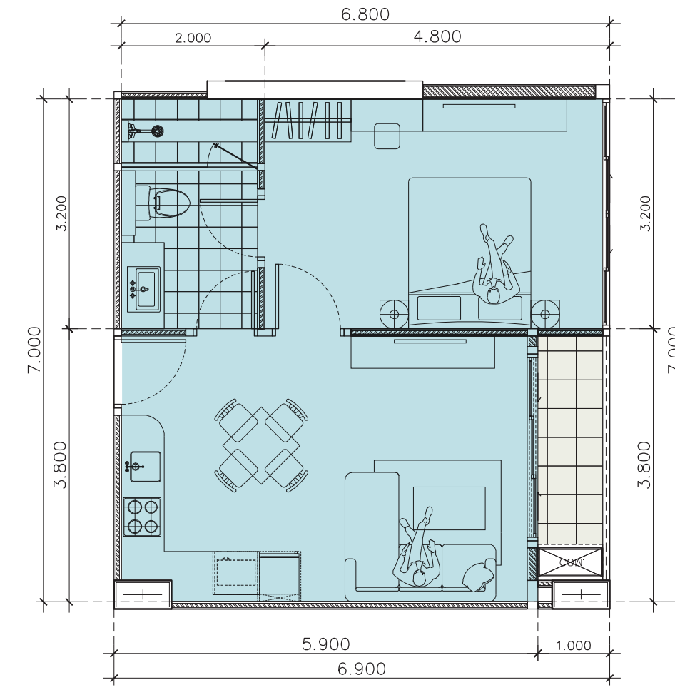
TYPE D 1 Bedroom DETAIL PLAN 47.24m 2
