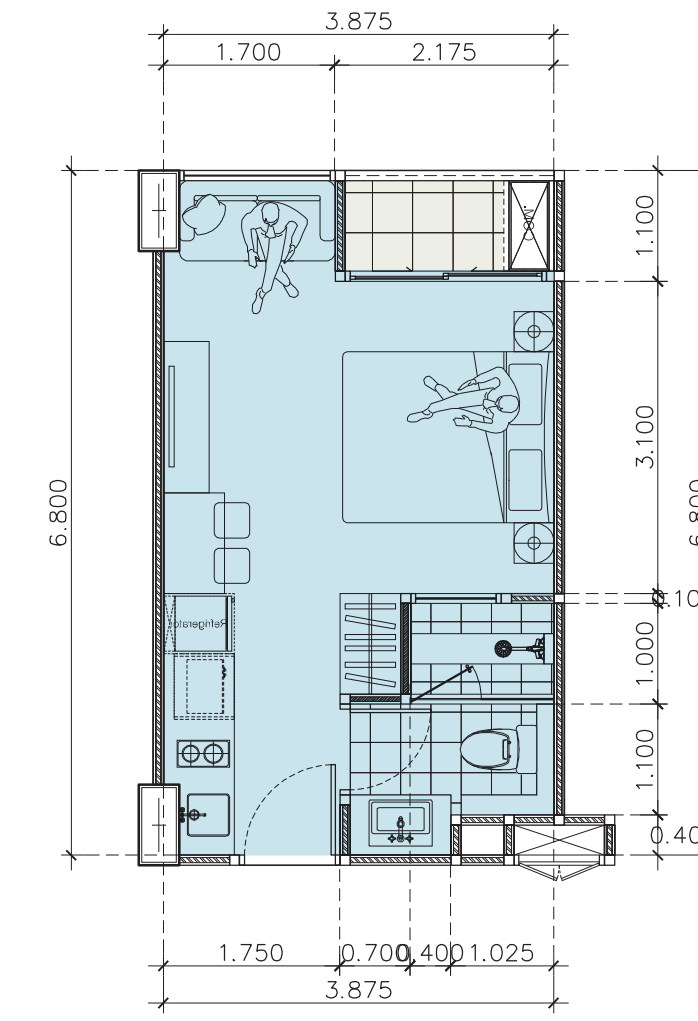
TYPE F Studio DETAIL PLAN 26.02m 2
