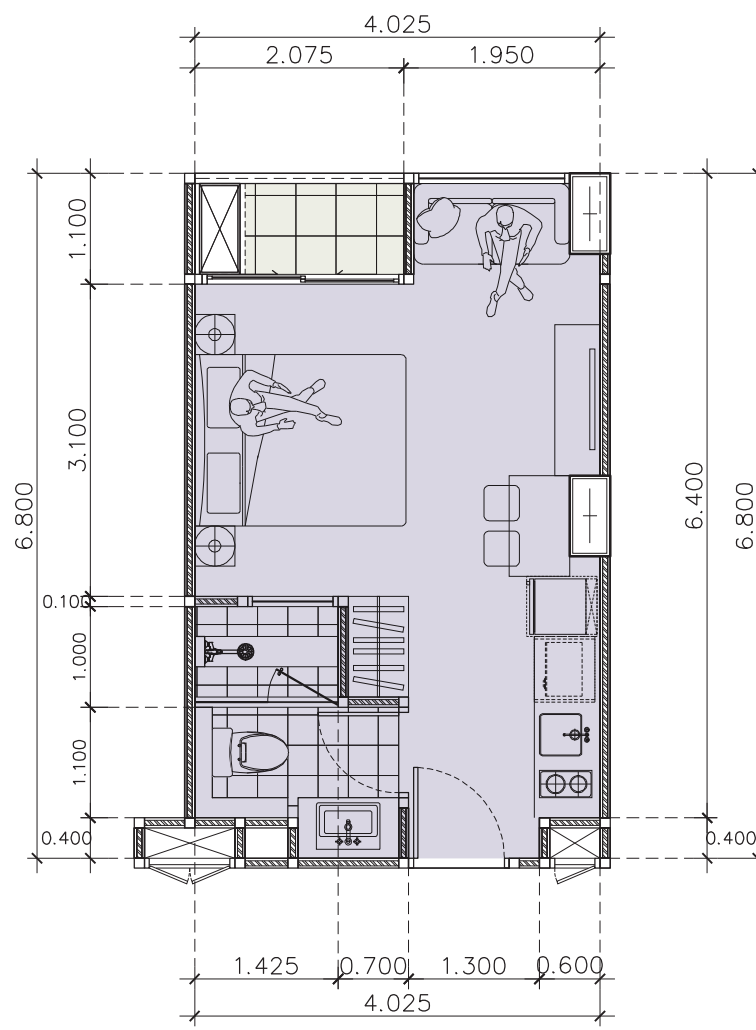
TYPE C Studio DETAIL PLAN 26.54m 2
