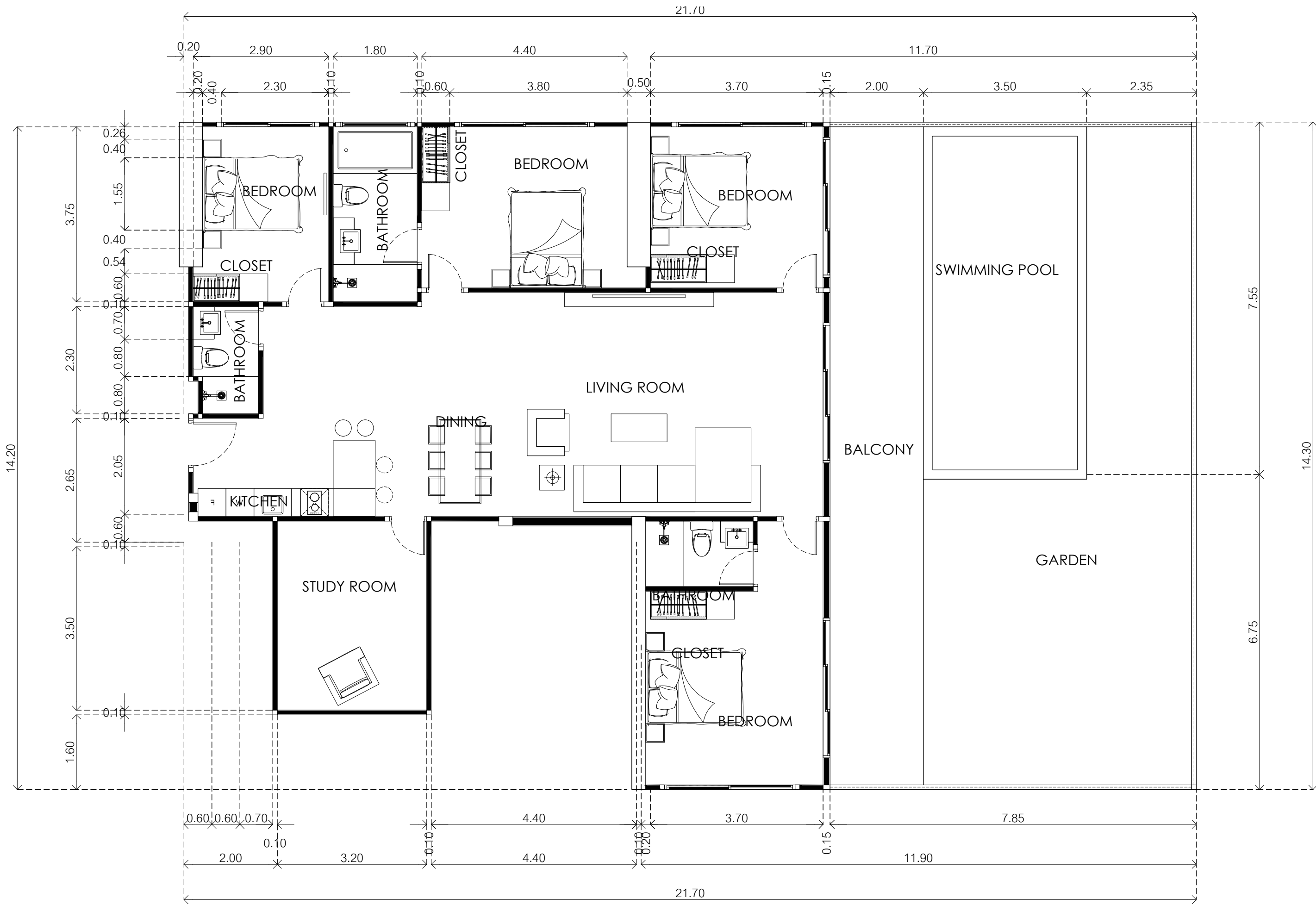
4BEDROOM 267.15 Scale 1:75
