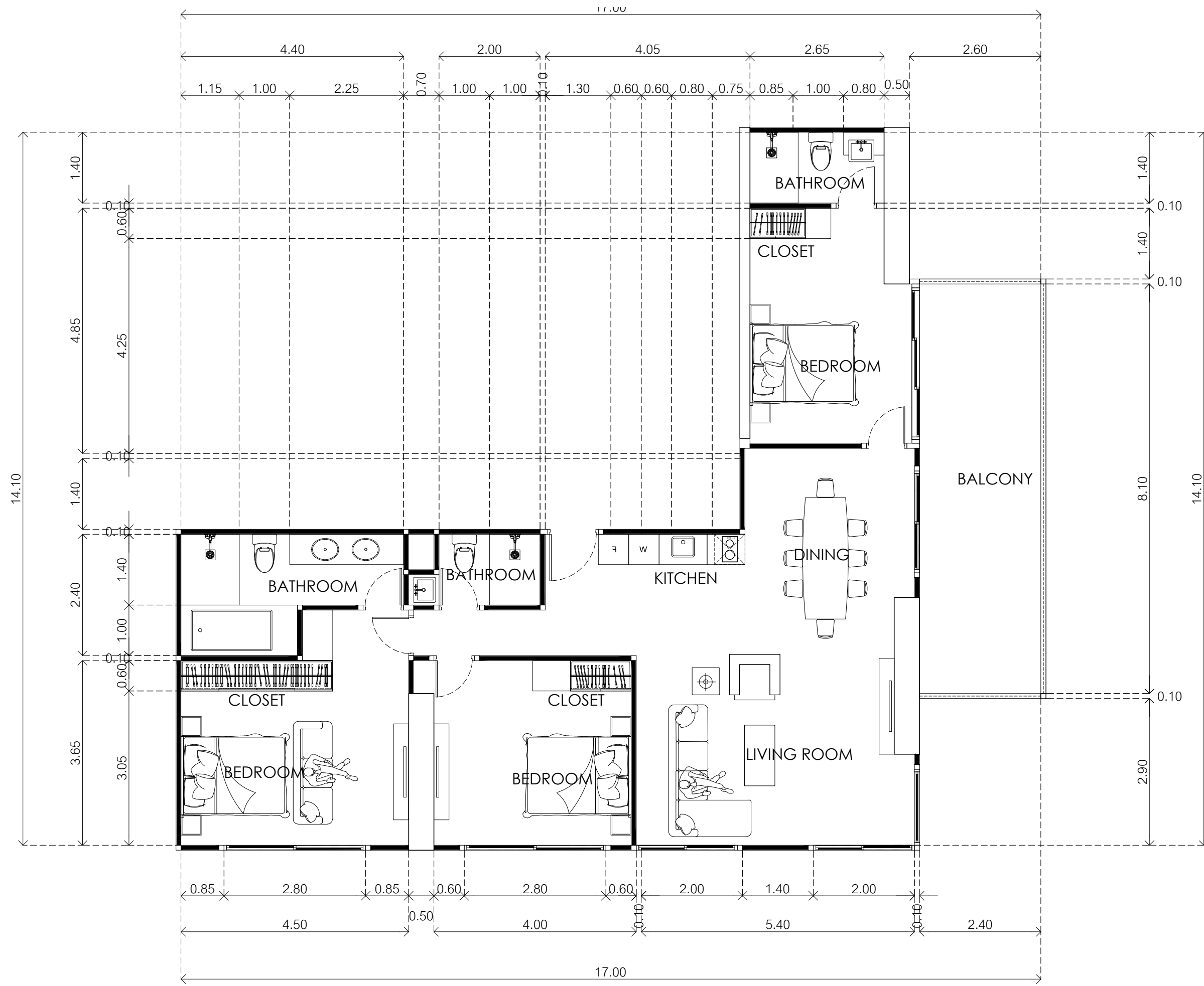
2BEDROOM 150.08 Scale 1:75
