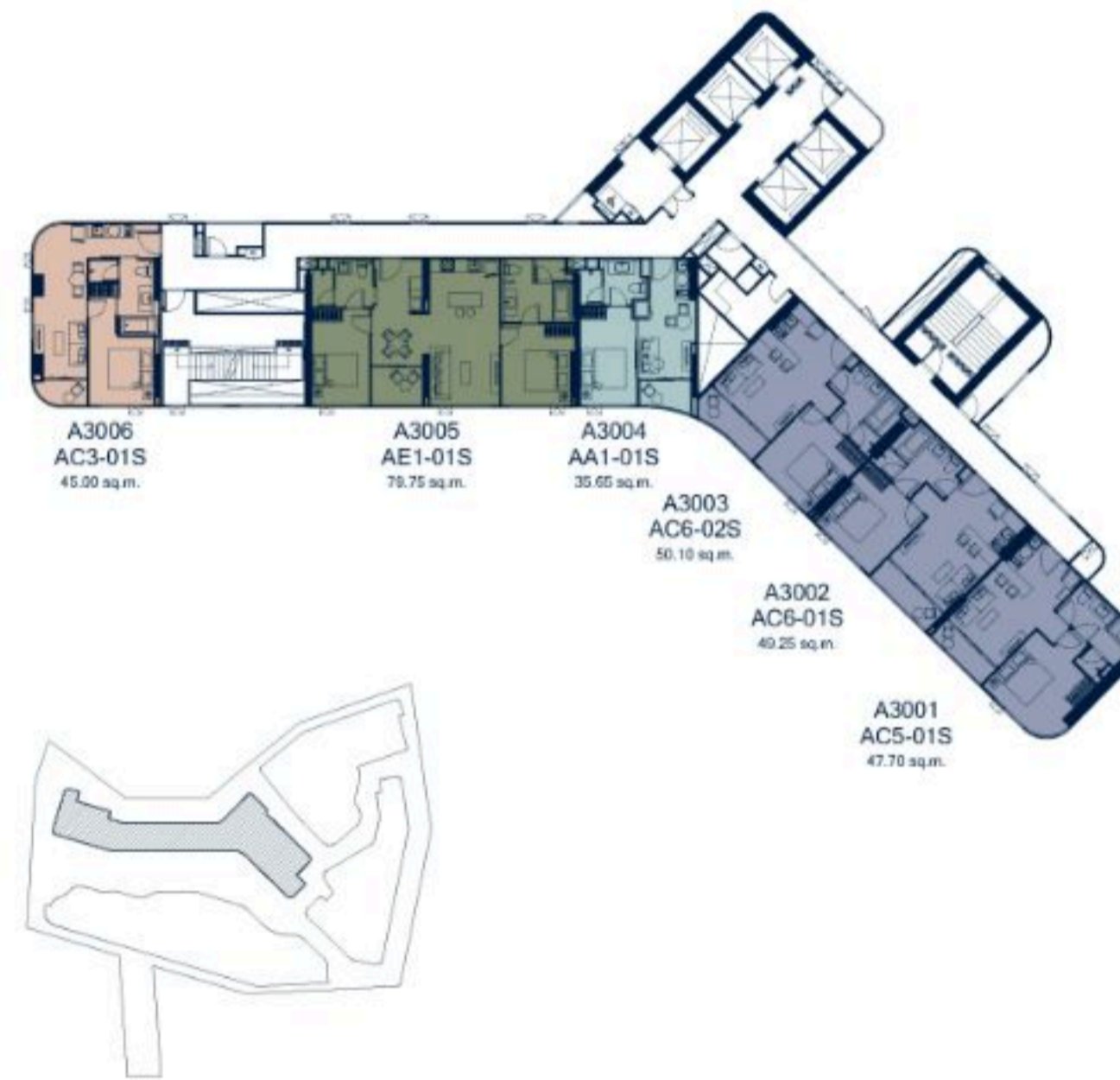
30 TH - 31 ST FLOOR PLAN
